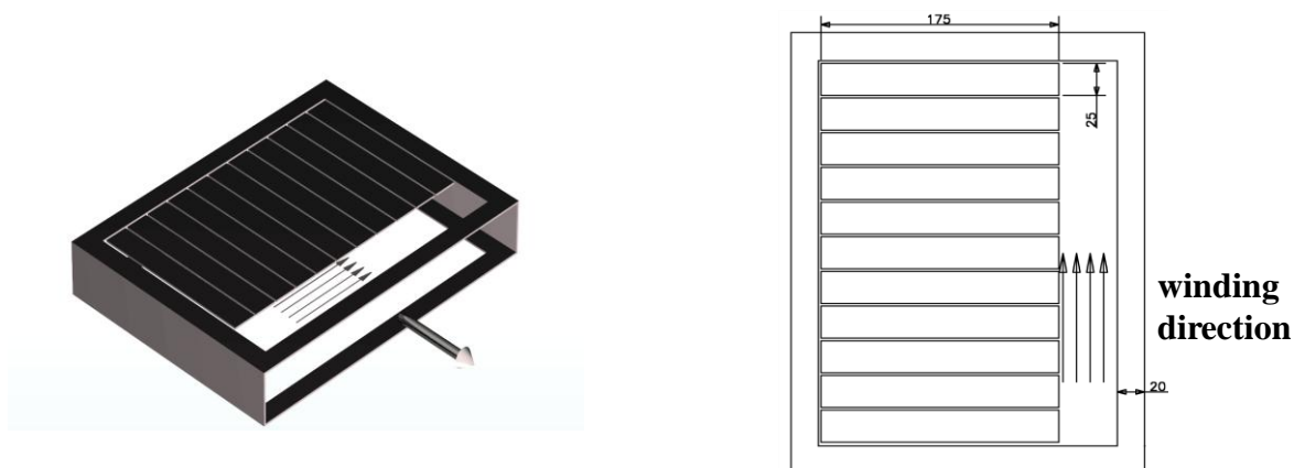
Figure 5. Basalt/epoxy panel sketch and transversal cutting direction of the specimens.
