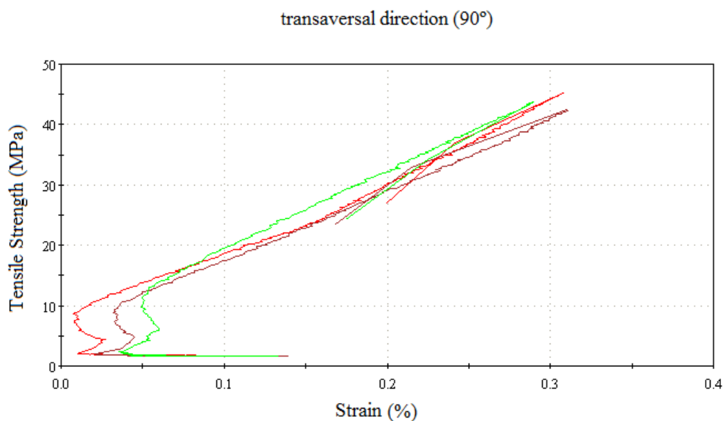
Figure 7. Tensile strength versus strain curve for basalt/epoxy composite specimens 1, 2 and 3 in the transversal direction ( 90^\circ ).
