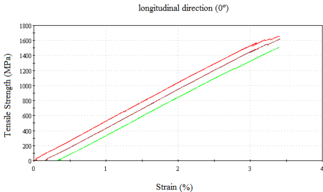
Figure 6. Tensile strength versus strain curve for basalt/epoxy composite specimens 1, 2 and 3 in the longitudinal direction ( 0^\circ ).
