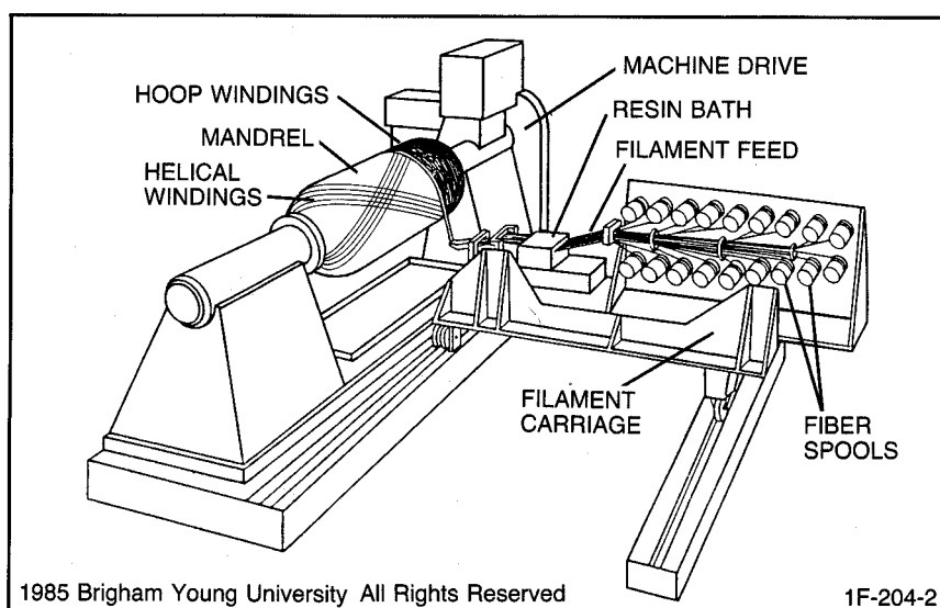
Figure 2. Filament winding machine [9].
