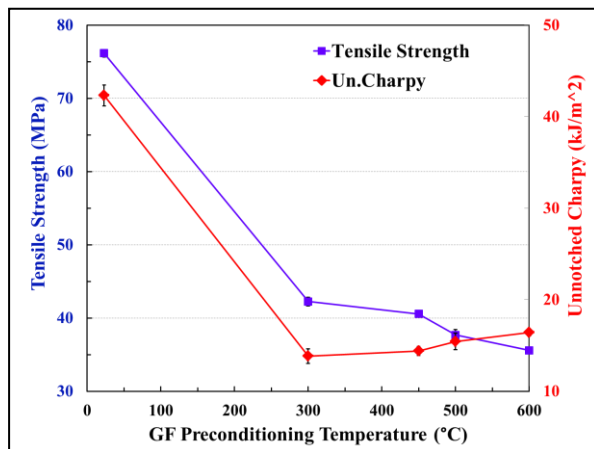
Figure 7: Effect of glass fibre heat treatment on composite performance
