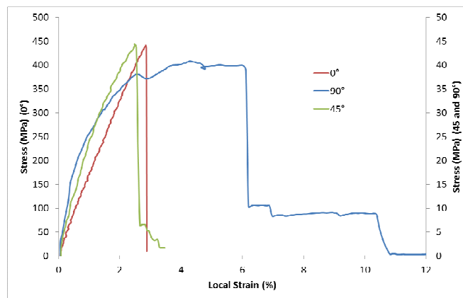
Figure 1. Quasi-static traction curves
