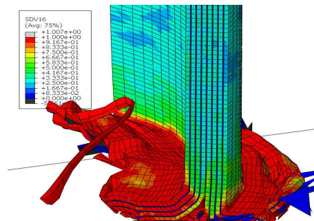
Figure 6. Simulation of drop-weight tower test
