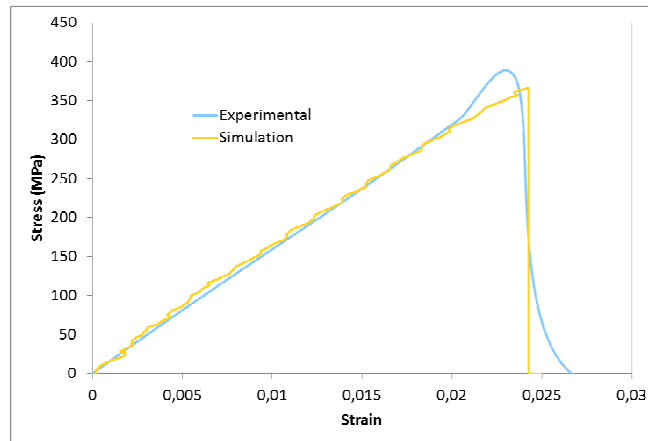
Figure 5. Experimental and simulation curves for quasi-static traction curve at 0°
