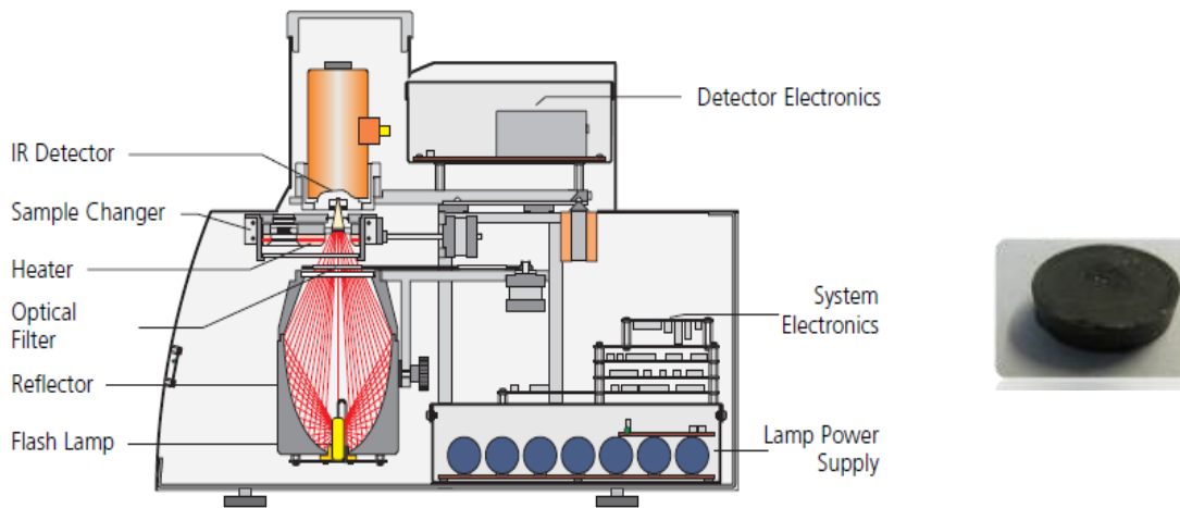
Figure 5. The NanoFlash system used in this work and the test specimen needed to make a measure.
