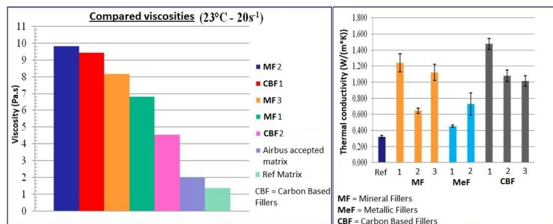
Figure 1. Viscosity and thermal conductivity for the model matrix charged with different particles
