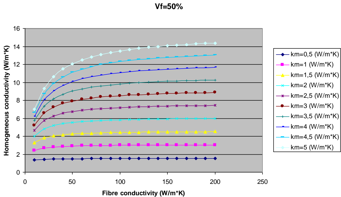
Figure 4. Homogeneous transverse conductivity function of the matrix and fibre conductivities at a 50% fibre ratio.
