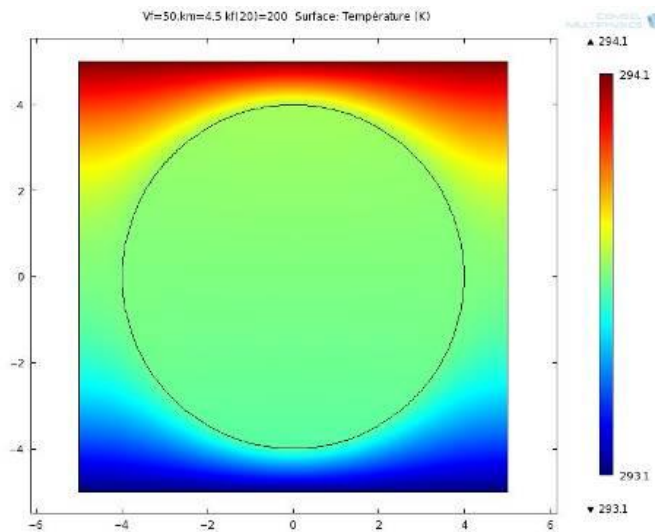
Figure 3. Elementary Representative Volume for the characterization of transverse thermal conductivity.
