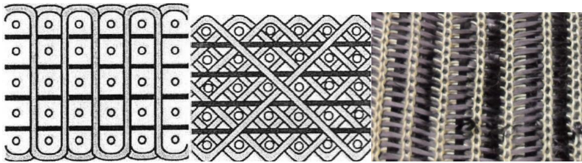
Figure 7. A 3D orthogonal Interlock, an Angled Interlock and a 3D textile developed by JTT Composite.
