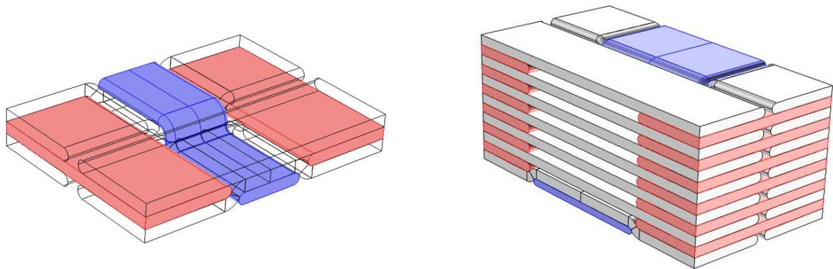
Figure 8. Example of 2 and 2.5D fibrous architectures used for composite thermal simulations.
