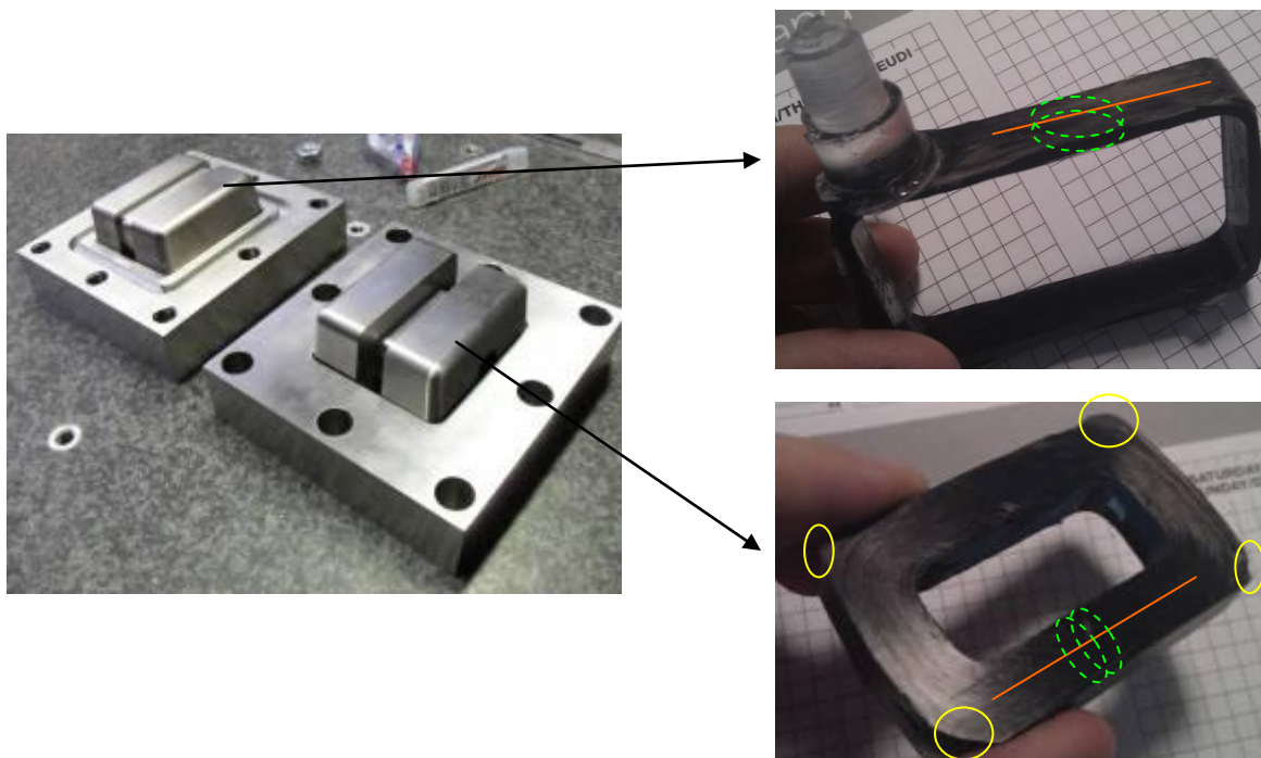
Figure 2. Modulable system to build the two type of test specimens
