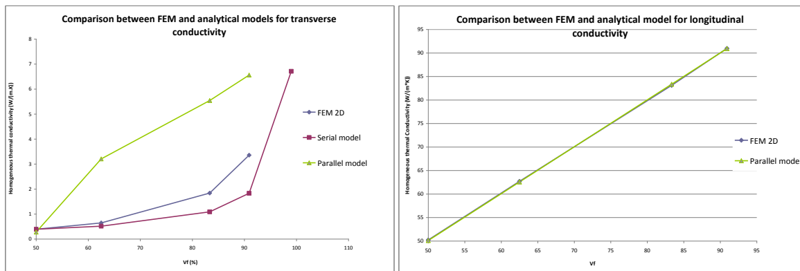
Figure 6. Comparison between FEM and analytical models for transverse and longitudinal conductivity
