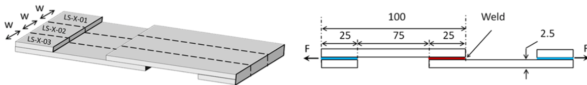
Figure 1. Dimensions of the used single lapshear specimen (in mm).
