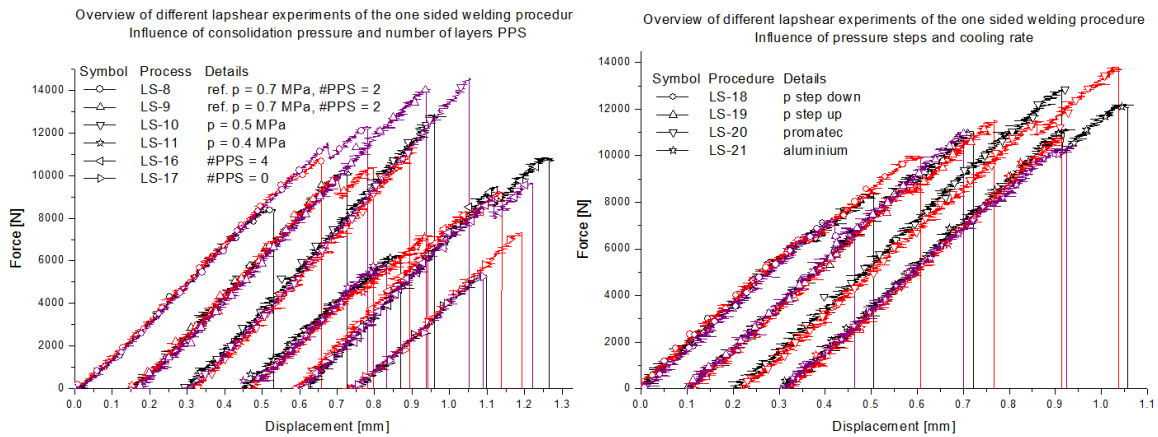
(a) Force versus displacement of the one sided welding procedure (part I). (b) Force versus displacement of the one sided welding procedure (part II).
